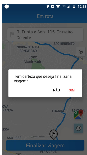
(b) Alerta
