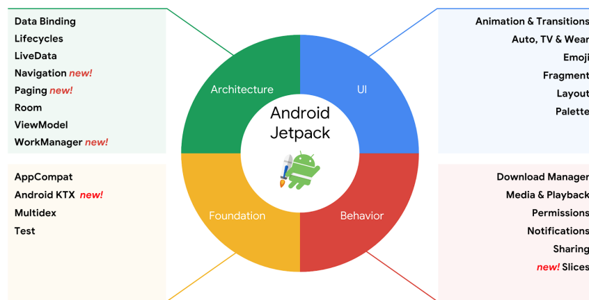
Figura 2 – Android Jetpack
