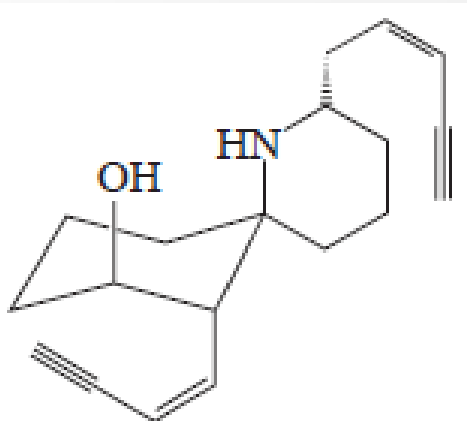
Histrionicotoxin
