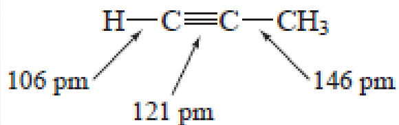
Propyne
