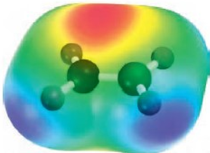
Ethylene
