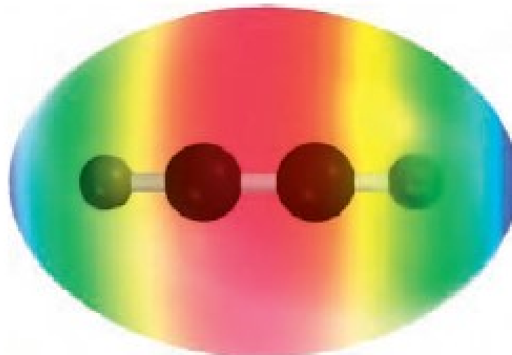
Acetylene
