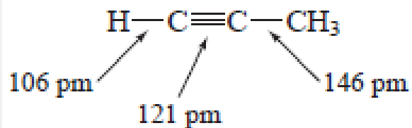
Propyne
