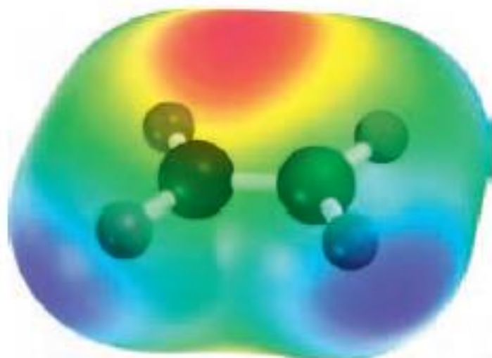
Ethylene
