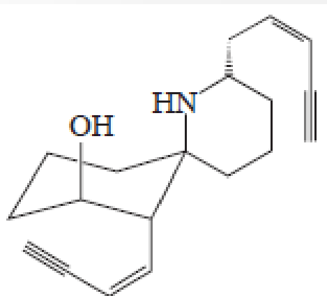
Histronicotoxin
