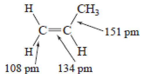
Propene
