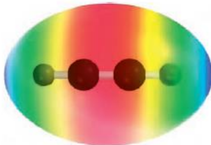
Acetylene
