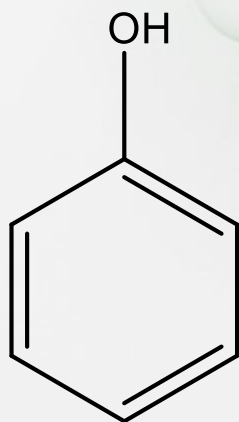
fenol
